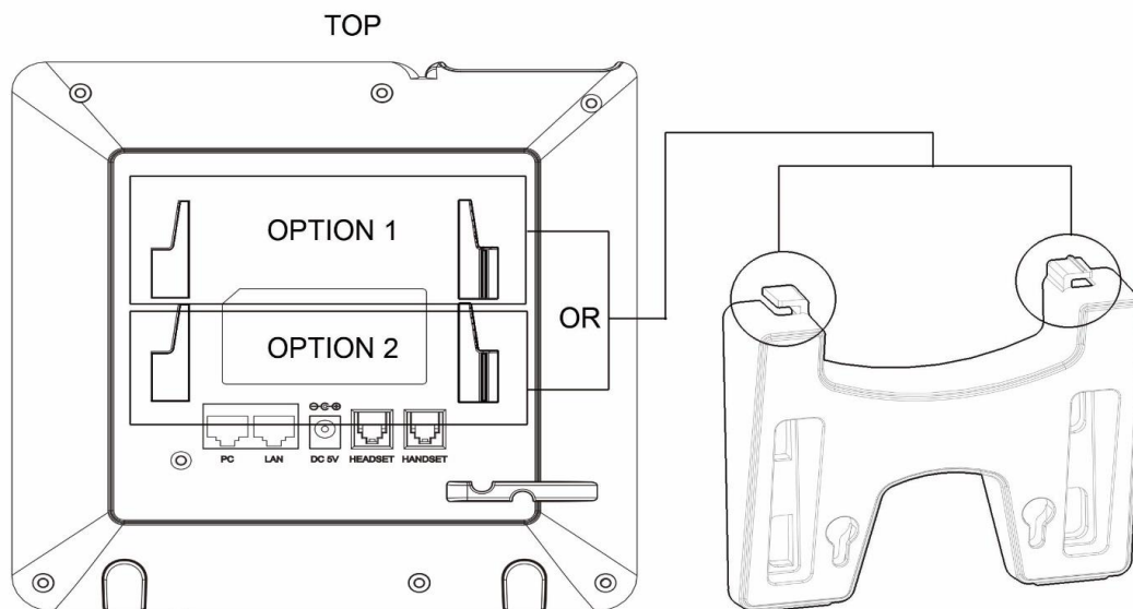
Figure 2: GXP16xx Stand Installation
